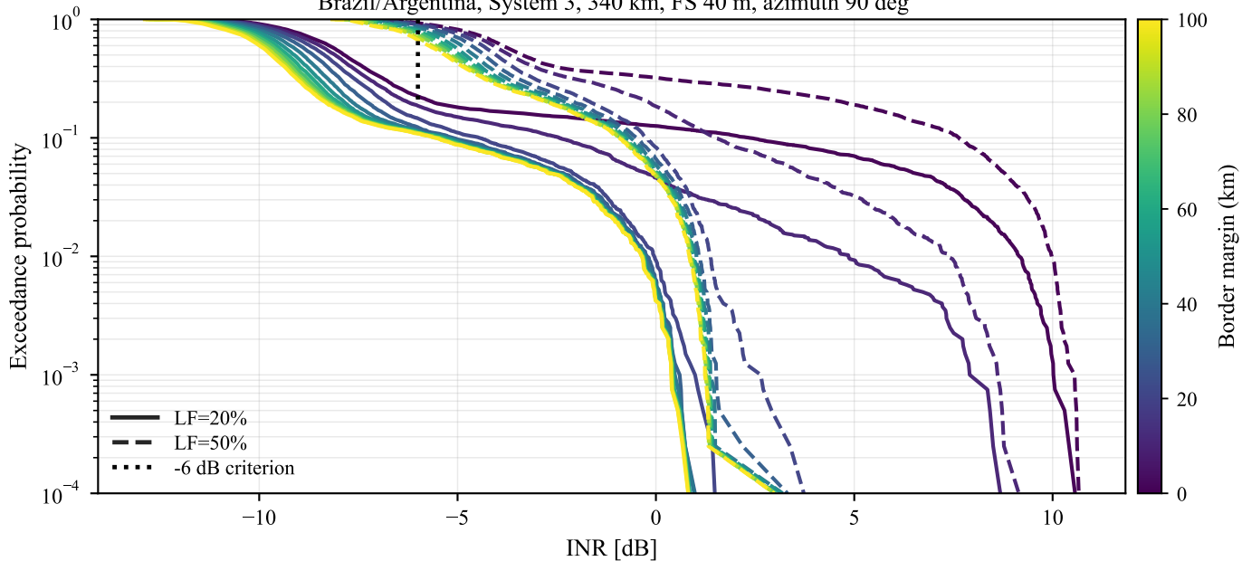
Brazil/Argentina, System 3, 340 km, FS 40 m, azimuth 90 deg
